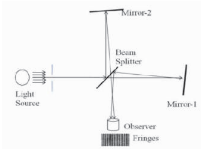
Fig 5: Schematic outline of Michelson's interferometer set up.
