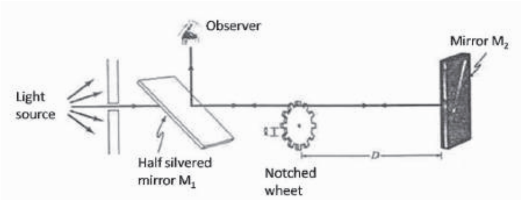
Fig 2: Schematic graph of Fizeau's trial setup.
