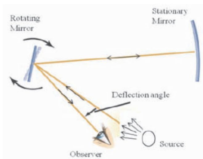
Fig 3: Scheme of Foucault's pivoting mirror setup.
