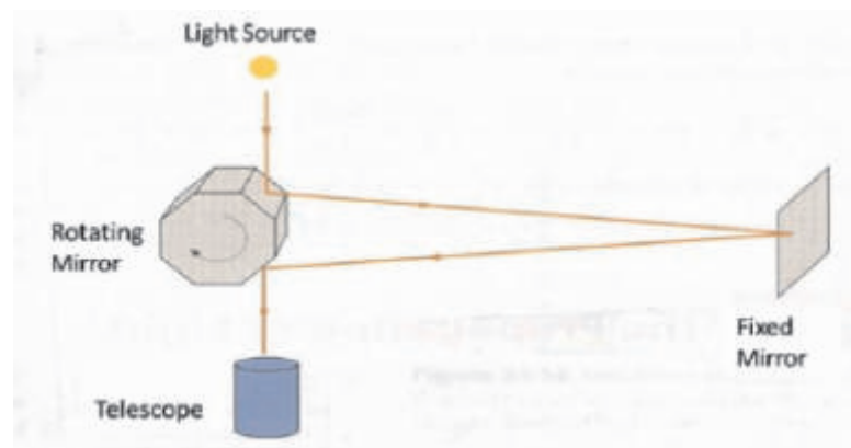
Fig 4: Schematic chart of Michelson's turning mirror set up.
