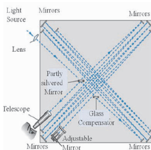
Fig 6: Scheme of Michelson-Morley interferometer set up.
