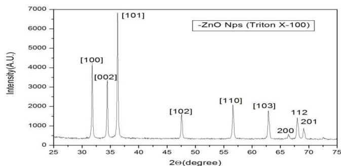
Fig.2 XRD pattern of ZnO powder prepared using reducing agent Triton X-100
