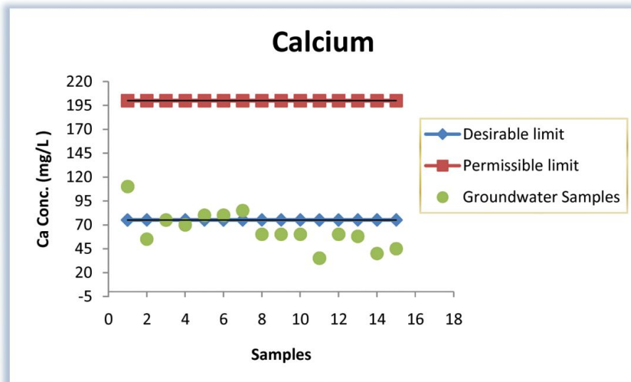
Fig.4 Distribution of Calcium
