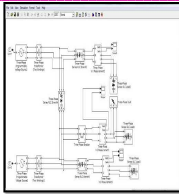
Figure 3 Power network in IEEE 14 bus network
